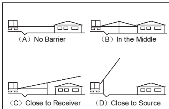
Figure1. How Noise Barriers Work
